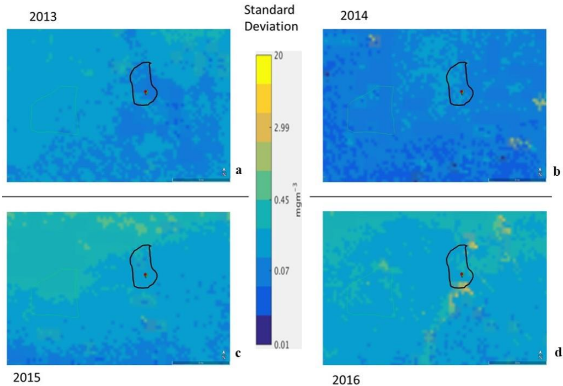
Figure 7. Standard deviation of chlorophyll at East Flower Garden Banks for June/July of 2013-2016. The temporal standard deviation of chlorophyll at each pixel for the eight 8-day time periods of June and July are shown for each year 2013 (a), 2014 (b), 2015 (c) and 2016 (d). A black line is used to delineate the East Flower Garden Banks boundary, and marker is located at the site of the mortality event.
